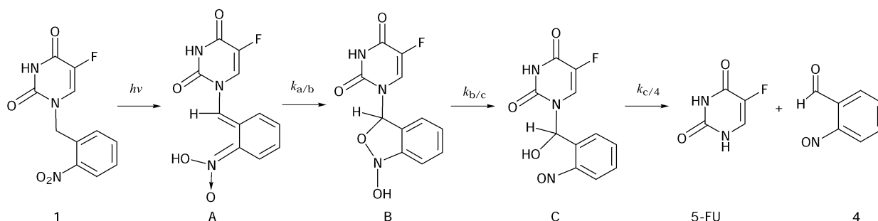
Scheme 2 Proposed mechanism of photoactivated 5-FU release from prodrug 1 in acetonitrile.
