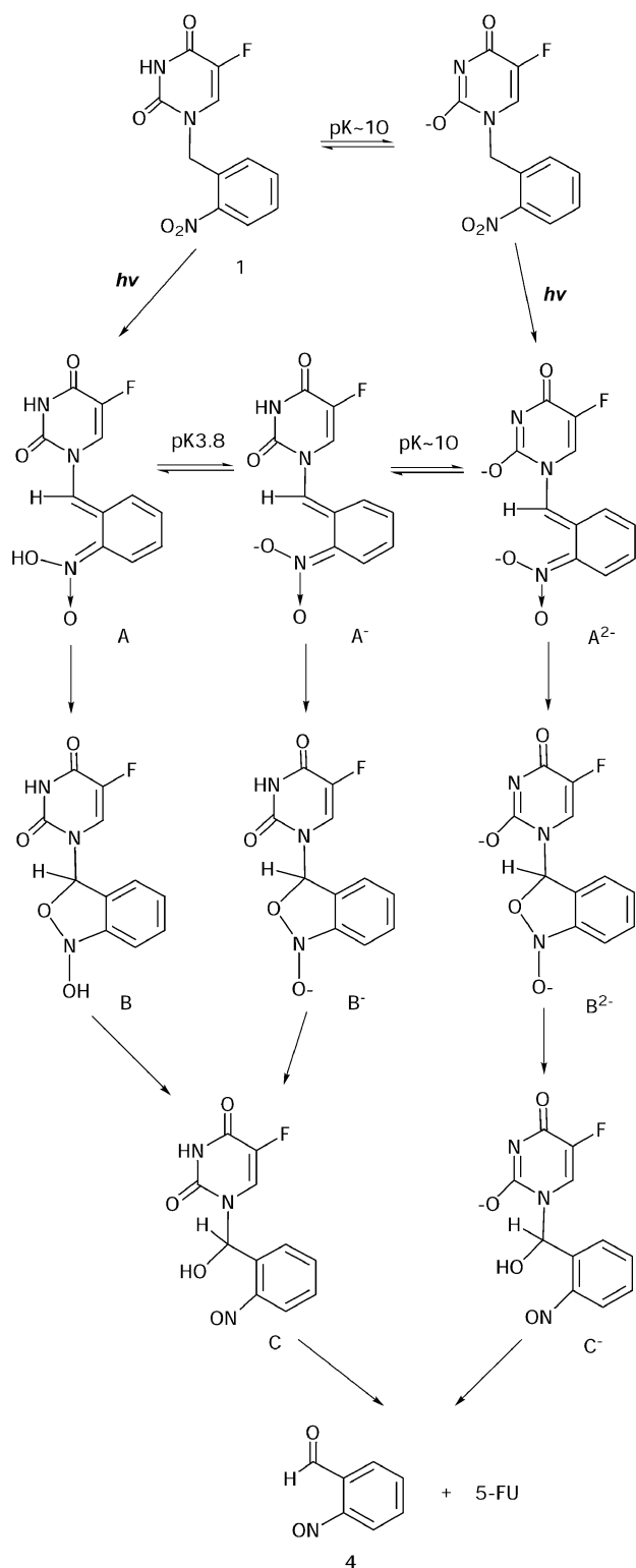
Scheme 3 Proposed mechanism of photoactivated 5-FU release from prodrug 1 in acetonitrile–H 2 O (2 : 1 v/v) solution.
