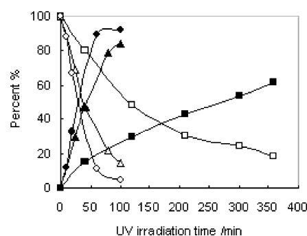
Fig. 1 Photolysis of prodrugs 1 and 2 in acetonitrile–H 2 O (2 : 1, v/v) and 3 in H 2 O at \lambda_{\text{ex}} = 365 nm: decrease of prodrugs ((○) 1 ; (△) 2 ; (□) 3 ) and 5-FU release from prodrugs ((●) 1 ; (▲) 2 ; (■) 3 ).
