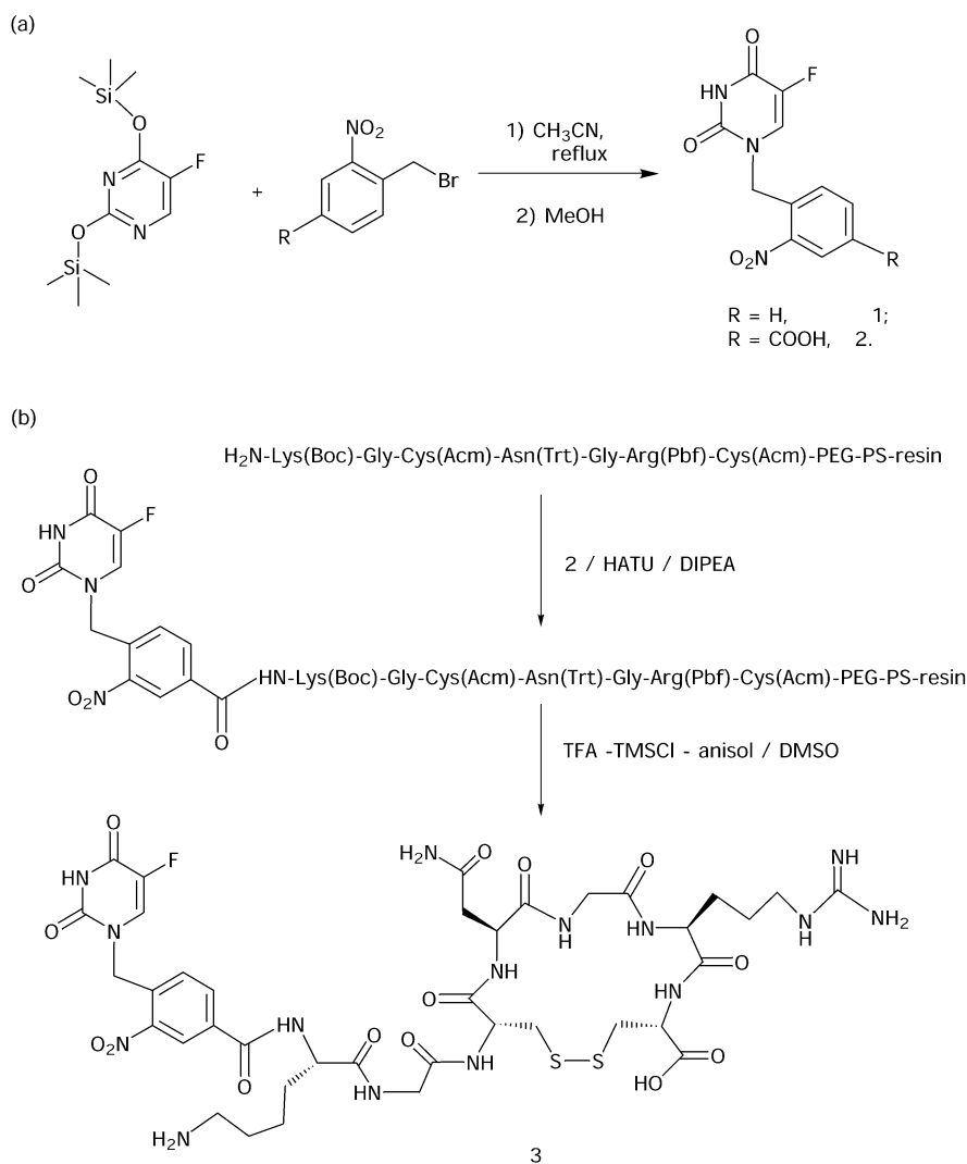
Scheme 1 (a) Syntheses of prodrugs 1 and 2 ; (b) synthesis of prodrug 3 .
